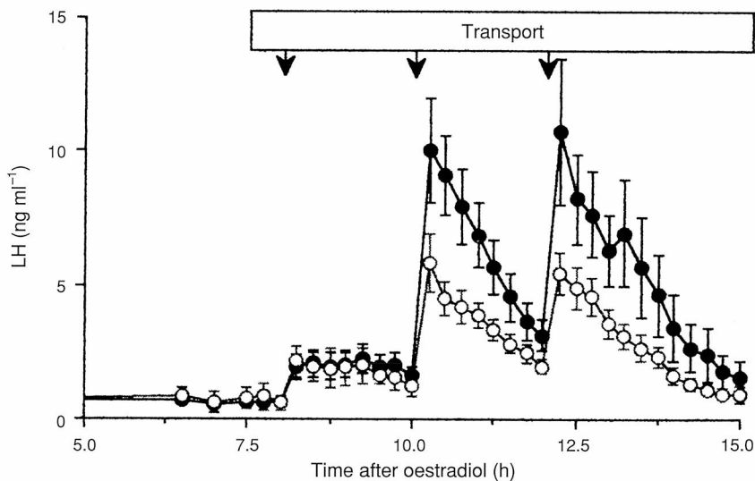
Fig. 4. Concentration of LH ( \pm SEM) in ewes in the breeding season treated with oestradiol benzoate (50 \mu\text{g} ) 24 h after prostaglandin synchronization with (○; n = 8 ) or without (●; n = 8 ) transport (duration indicated by the horizontal bar □) and 500 ng GnRH administered at times shown by the arrows. In control ewes not given GnRH, the concentration of LH did not exceed 1.5 \text{ ng ml}^{-1} .
